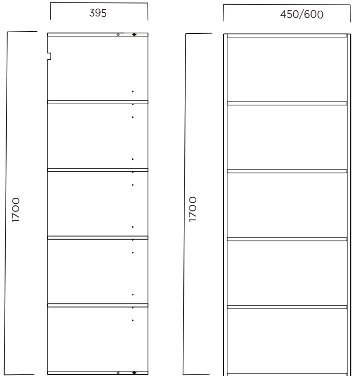
Wall-hung Tower unit with shelves W600xH1700xD395 W450xH1700xD395
