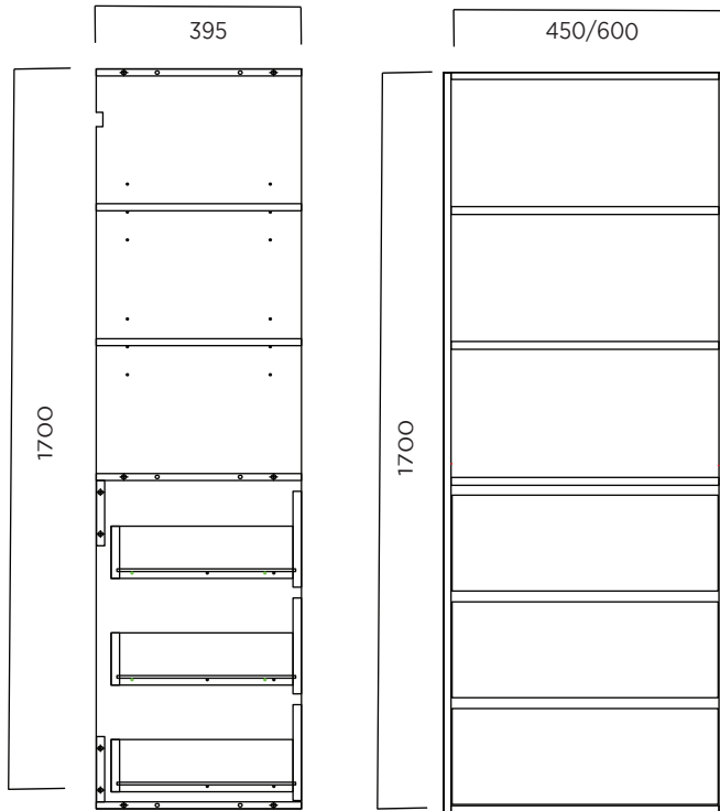
Wall-hung Tower unit with three drawers W600xH1700xD395 W450xH1700xD395
