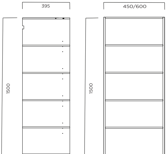
Wall-hung Tower unit with Shelves W600xH1500xD395 W450xH1500xD395
