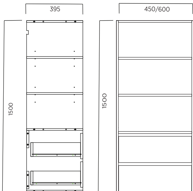
Wall-hung Tower unit with two drawers W600xH1500xD395 W450xH1500xD395
