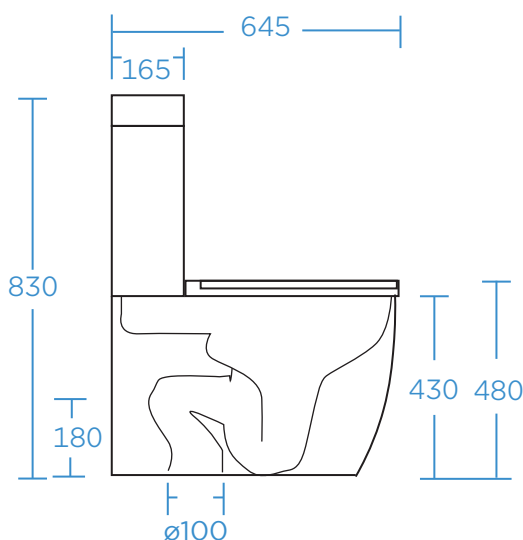
SIDE VIEW +/-5mm
